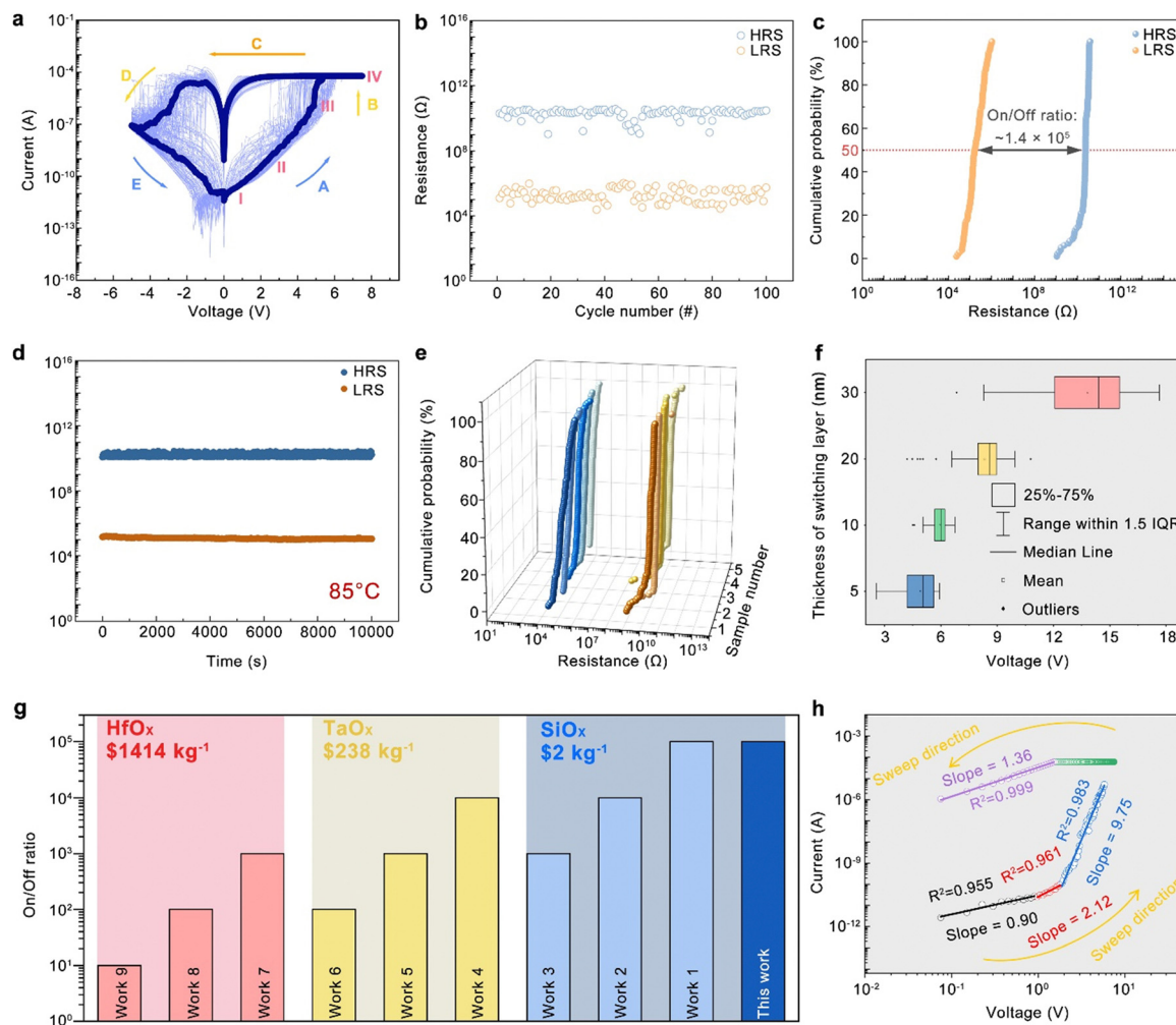
Fig. 2 (a) I – V characteristics of the Pd/SiO 2 (5 nm)/P + -Si memristor in semi-log scale, where arrows, labeled in alphabetical order, indicate HRS, SET, LRS, RESET, and HRS, respectively. (b) Endurance graph for 100 cycles, two distinct HRS and LRS remain without damping. The resistance values at HRS and LRS are recorded at a read voltage of 0.3 V. (c) Statistical distribution of resistance at HRS and LRS, from which the on/off ratio is extracted to be \sim 1.4 \times 10^5 at a cumulative possibility of 50%. (d) The retention characteristics of 5 nm SiO 2 memristor at LRS and HRS, examined at 85 °C, exhibit reasonably good performance. (e) The statistical distribution of R HRS and R LRS for 5 different devices. The on/off ratios were obtained by using the same method in (b). Similar high on/off ratios of \sim 10^5 are obtained from all the devices. (f) Statistical distribution SET voltages for different thicknesses of SiO 2 switching layers. (g) Comparison of the on/off ratio of the present study with those from the literature. (h) Analysis of electric transport processes of the SiO 2 -based memristor in log–log scale.
